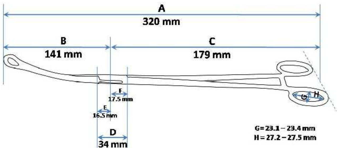
Figure: Dimensions of the PPIUCD insertion forceps
