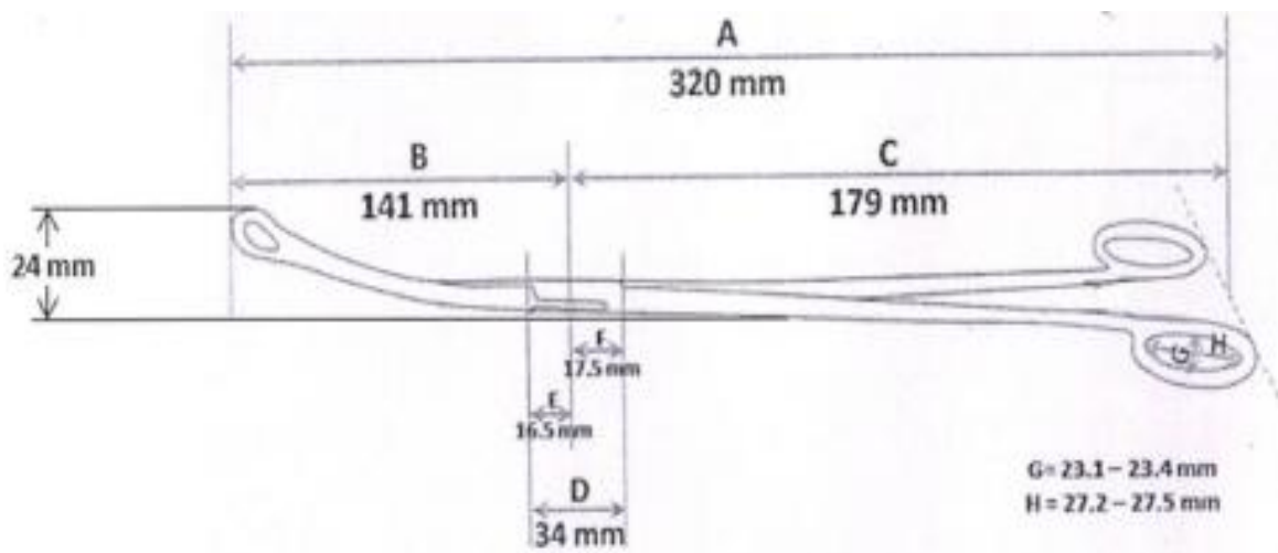
Figure: Dimensions of the PPIUCD insertion forceps
